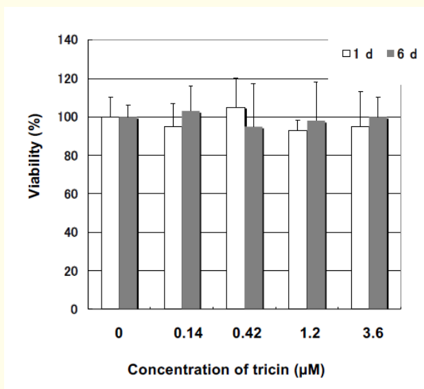
Figure 6: Direct toxicity of Tricin upon nursing cell.
