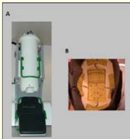
Figure 1: A) The 122-channel MEG system. B) The pT-TMS electronic device.
